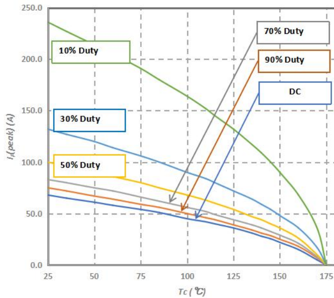
Fig.7-Current Derating
